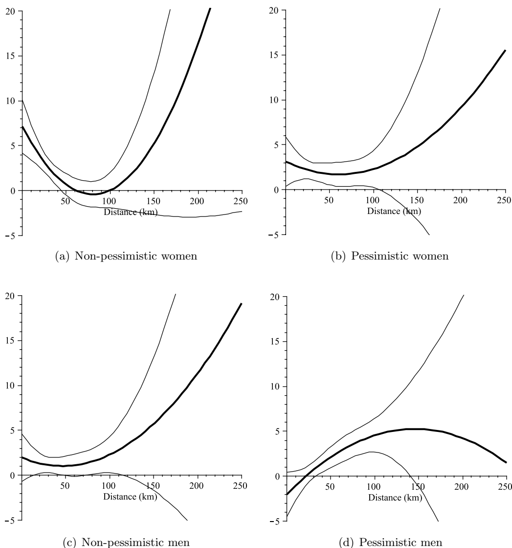
Figure 1: Marginal willingness to pay for increased coverage with respect to distance (measured in km) from nuclear power plant, in US$ per year. The thin lines show the 95 percent confidence intervals calculated with the Delta method.
